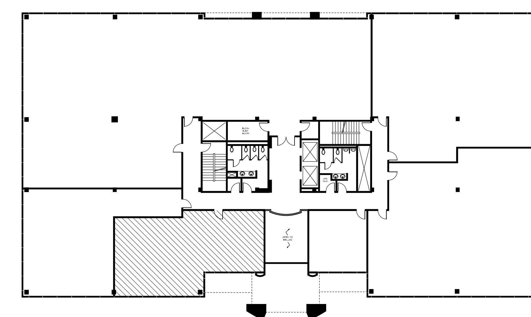
KEY PLAN
