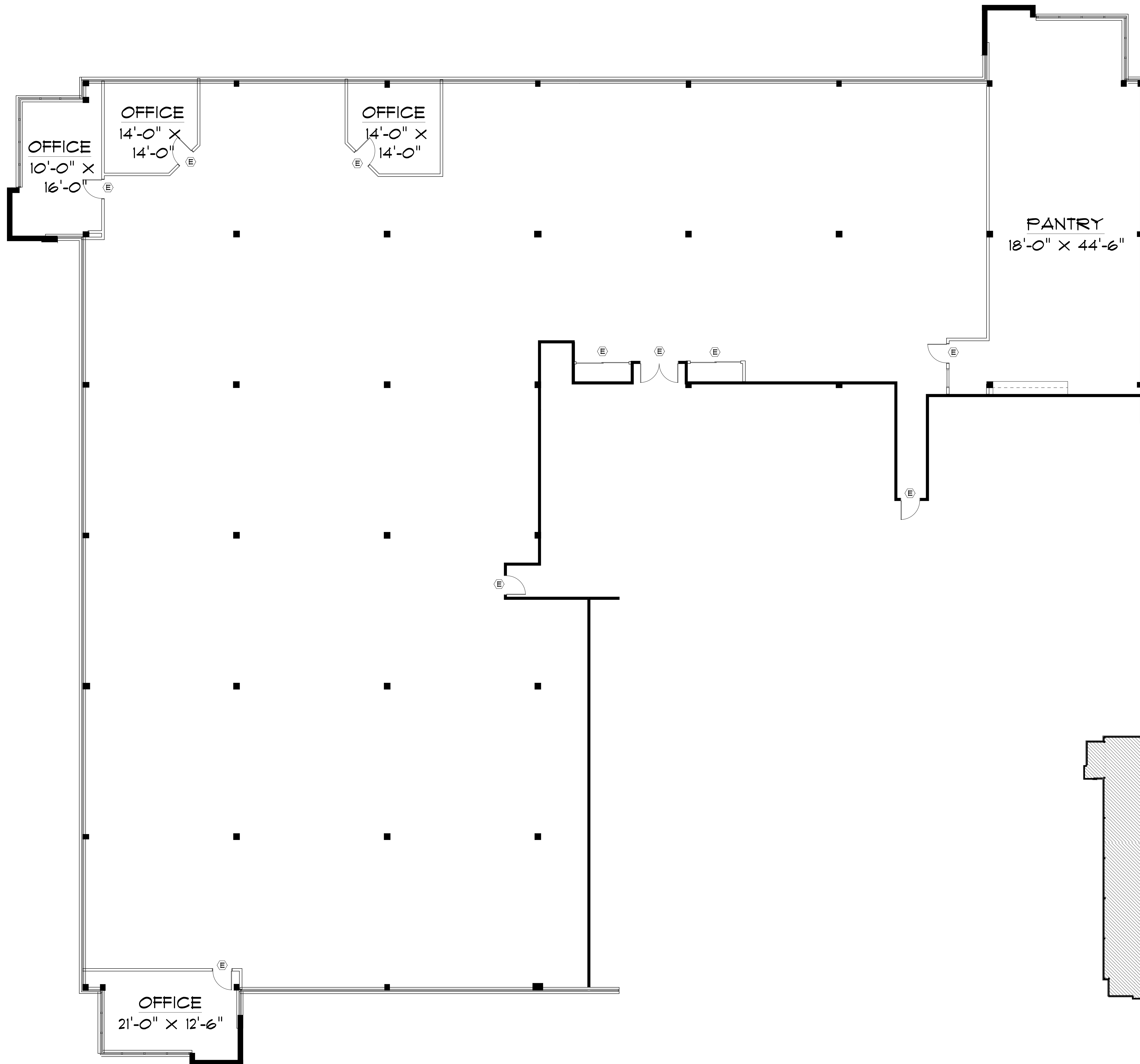
KEY PLAN
