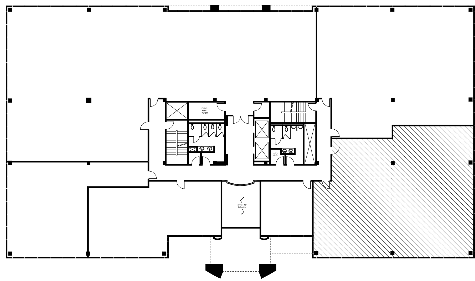
KEY PLAN
