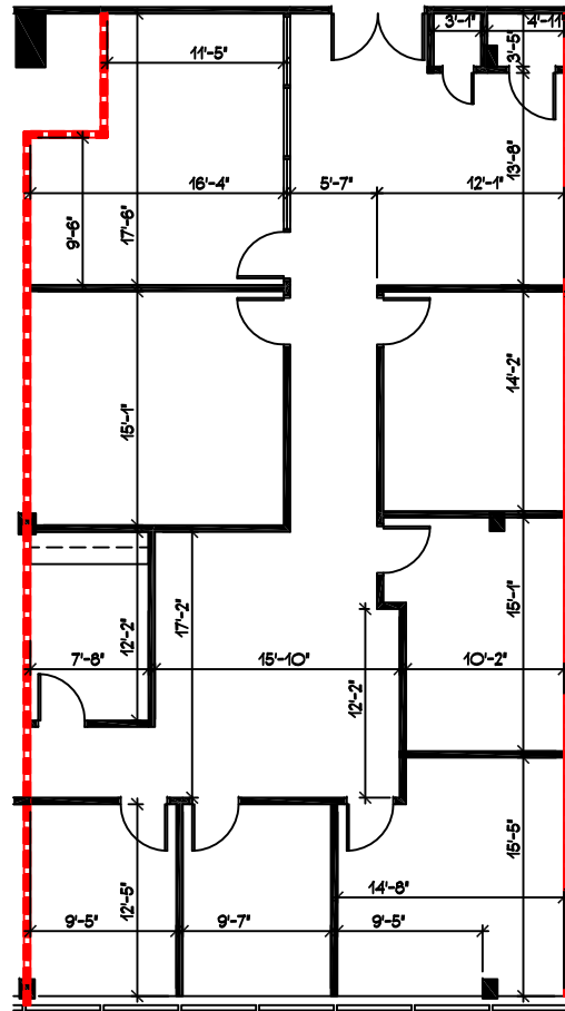
SECOND FLOOR -SUITE # 203 - 2,700 RSF
