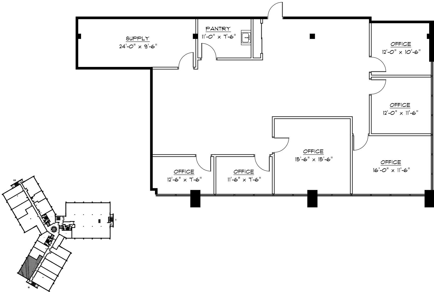
THIRD FLOOR - BLDG 2 - SUITE 354 - 2,807 SQ. FT.
